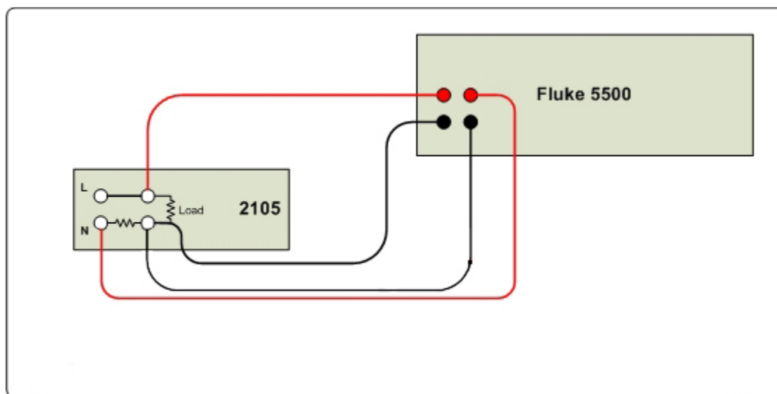
Figure 6-1 | DC Connections
